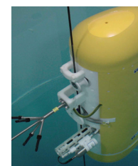
Older version 52-MP on McLane Moored Profiler
